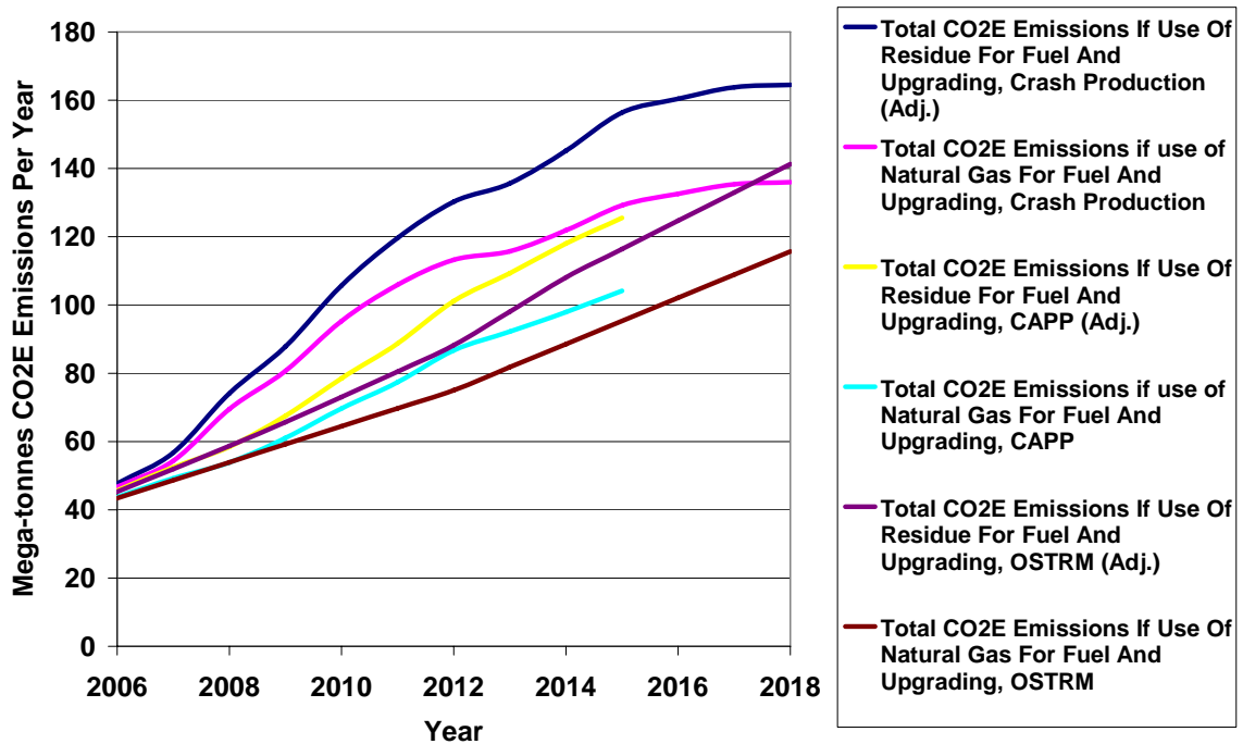
Fig. 8. The figure illustrates potential CO 2 E emissions from three oil sands production forecasts; The Crash Program Production Forecast, the CAPP-forecast and the OSTRM-forecast. For each of the three forecasts, two CO 2 E-emissions forecasts are presented, one when natural gas has been assumed as the primary fuel for heat and upgrading and a scenario when bitumen gradually replaces the need of natural gas. The latter is referred to as Adj. (Adjusted).
