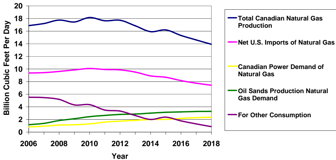
Fig 7. The curve named For Other Consumption illustrates a probable future increasing scarcity of natural gas for other consumption in Canada. This is likely to imply constant or even higher natural gas prices in the future. High prices will increase the uncertainty for primarily in situ oil sands investments and might dampen the will to invest, thus slowing the development pace for the Canadian oil sands industry.
